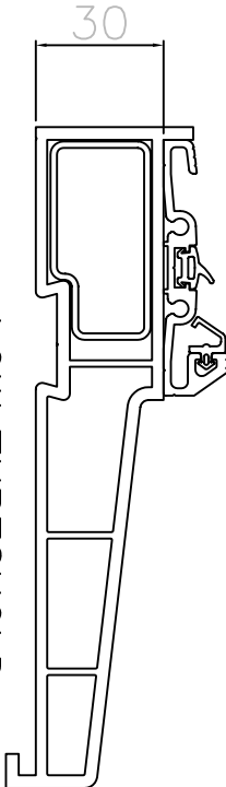
LOW THRESHOLD ON WITH CILL CILL SIZES 85MM,155MM,180MM
