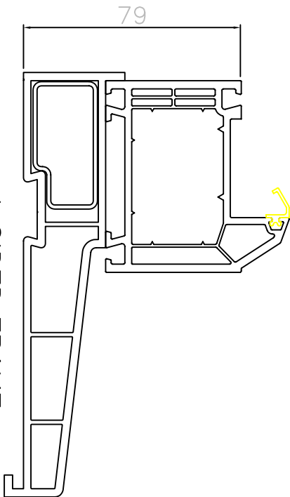
4 SIDED FRAME WITH CILL (ALSO AVAILABLE WITHOUT CILL)
